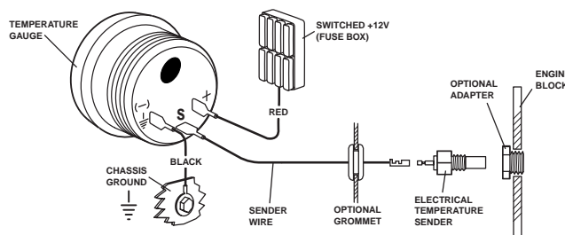
Figure 5. Electric Water Temperature Gauge Connections
